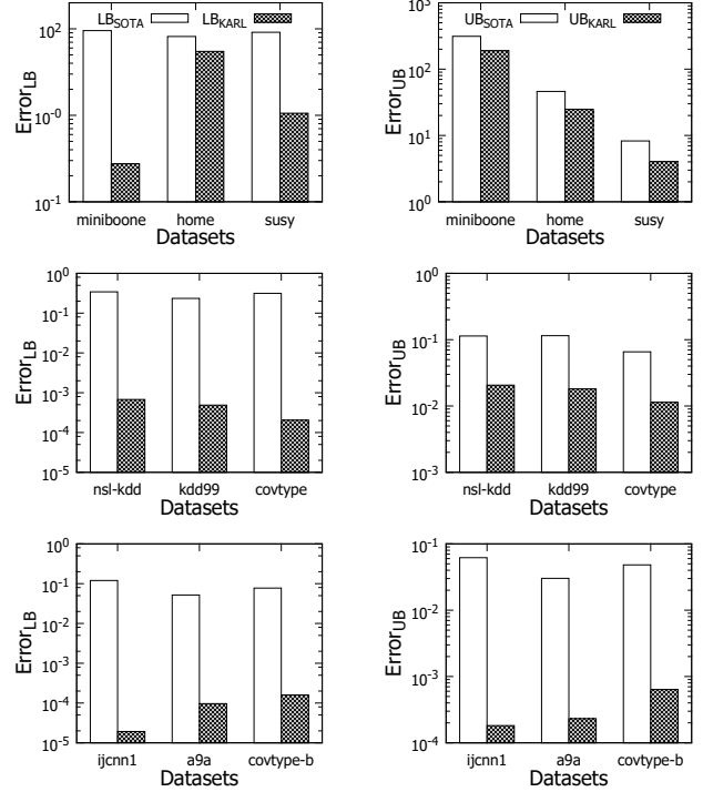
Figure 13: Error_{LB} and Error_{UB} for Type-I, II and III queries
